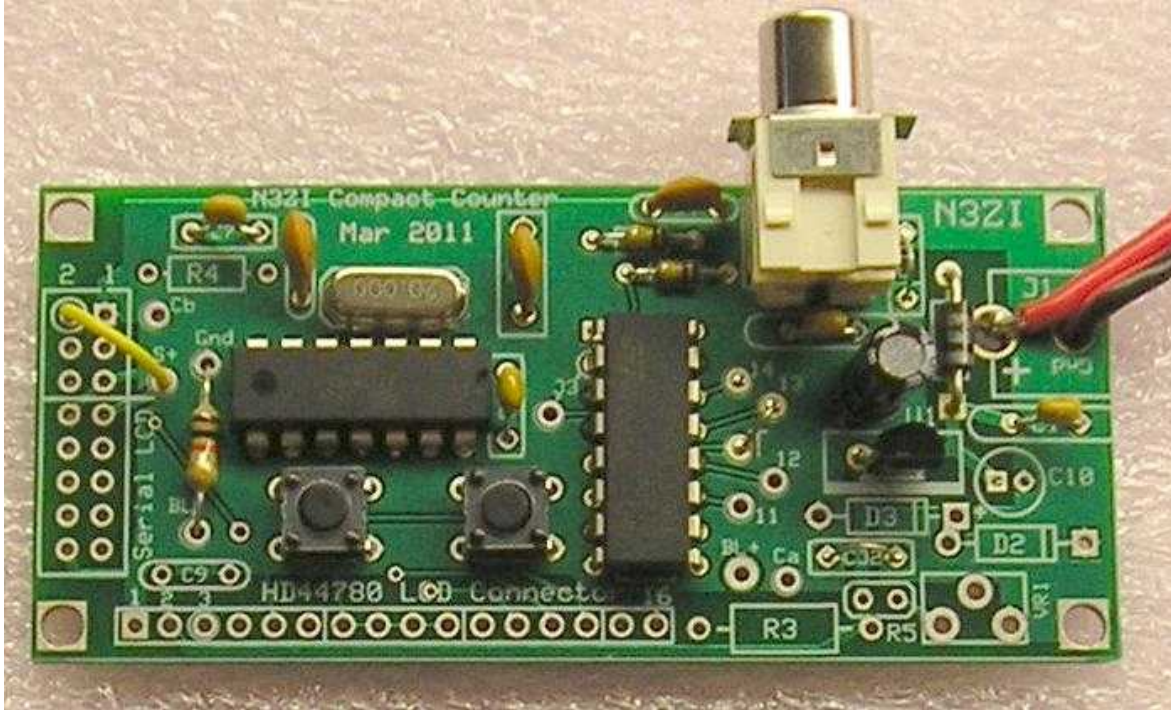
Full kit properly assembled and configured for Standard Serial LCD (LCD Not yet connected)
