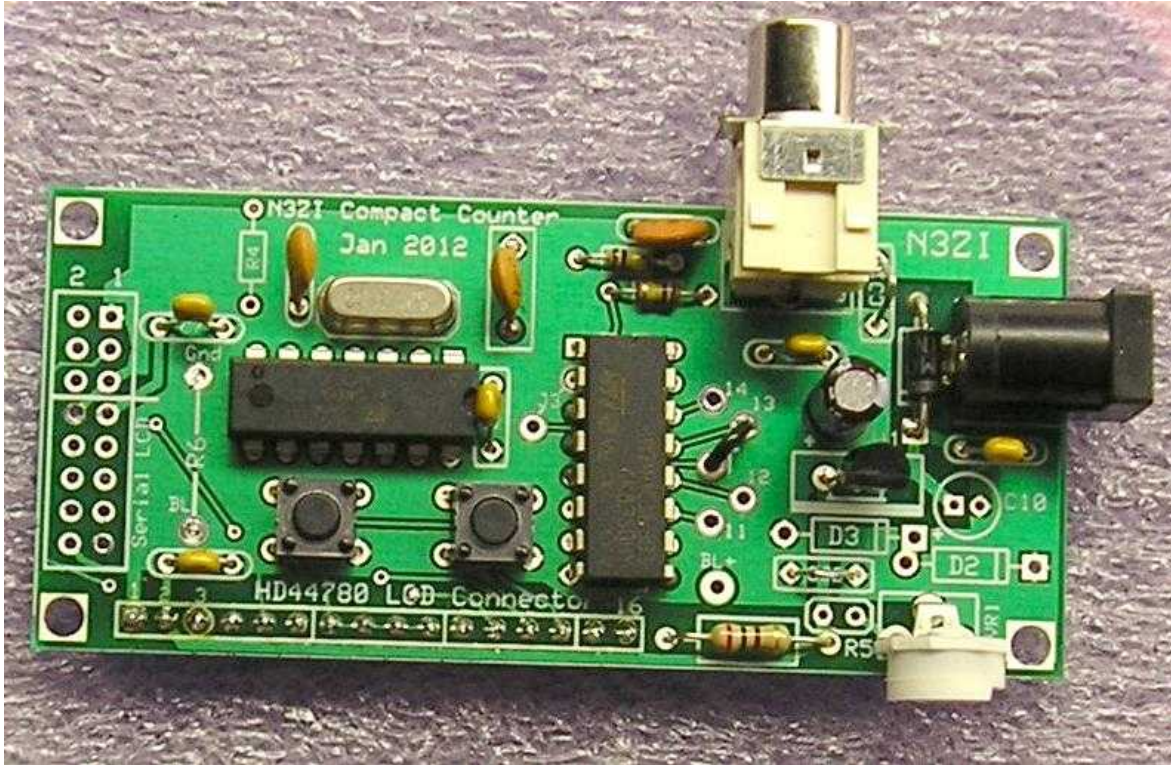
Kit properly assembled and configured for Blue Backlit LCD
